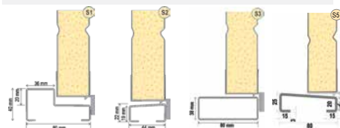
Side doors threshold
